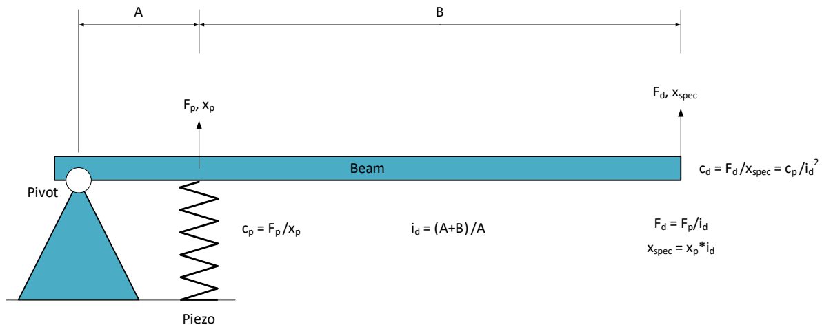
Fig 2: Relation between scanner motion range and drive stiffness (no load).
